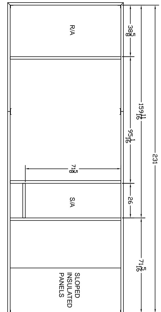
TOP VIEW
