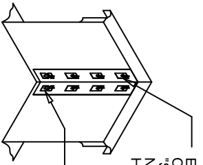
CURB CORNER SECTION (U.S. PATENT) (#5465533)
